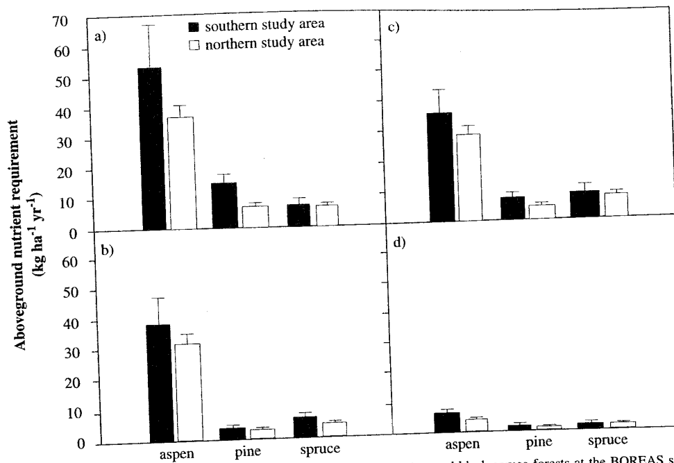
FIGURE 3. Annual above-ground nutrient requirement for trembling aspen, jack pine, and black spruce forests at the BOREAS southern and northern study areas. All values are in \text{kg ha}^{-1} \text{yr}^{-1} . Bars are the means of four plots \pm SE.
