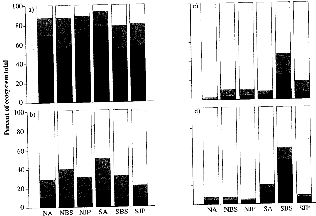
FIGURE 1. Percent nutrient distribution for trembling aspen, jack pine and black spruce forests at the BOREAS northern study area (NA, NBS, NJP) and southern study area (SA, SBS, SJP). Figure a-d are for carbon, nitrogen, calcium, and magnesium, respectively. For all panels the four components from top to bottom are mineral soil, forest floor, wood (stem, branch, and coarse roots), and foliage. Fine roots and understory are excluded, but comprised < 2% of the total ecosystem organic matter budget.
