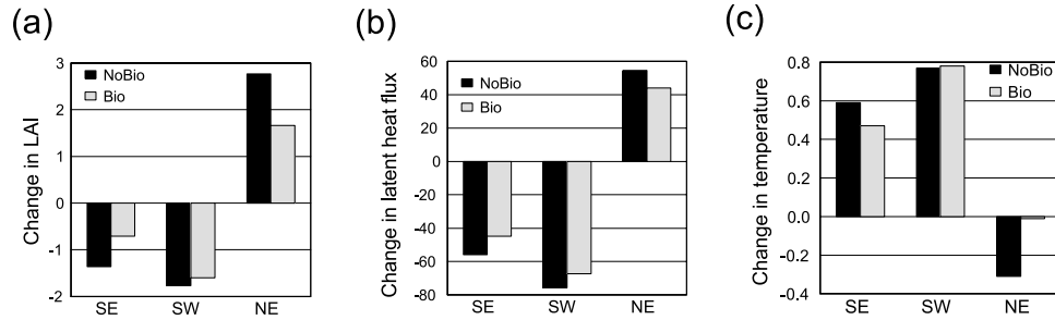
Figure 2. Simulated change (relative to CC ) in (a) LAI; (b) latent heat flux ( W m^{-2} ); (c) temperature ( ^{\circ}C ) for the NoBio (black bars) and Bio (lightly shaded bars) for Southeast (SE), southwest (SW) and northeast (NE) Australia (see Figure 1).
